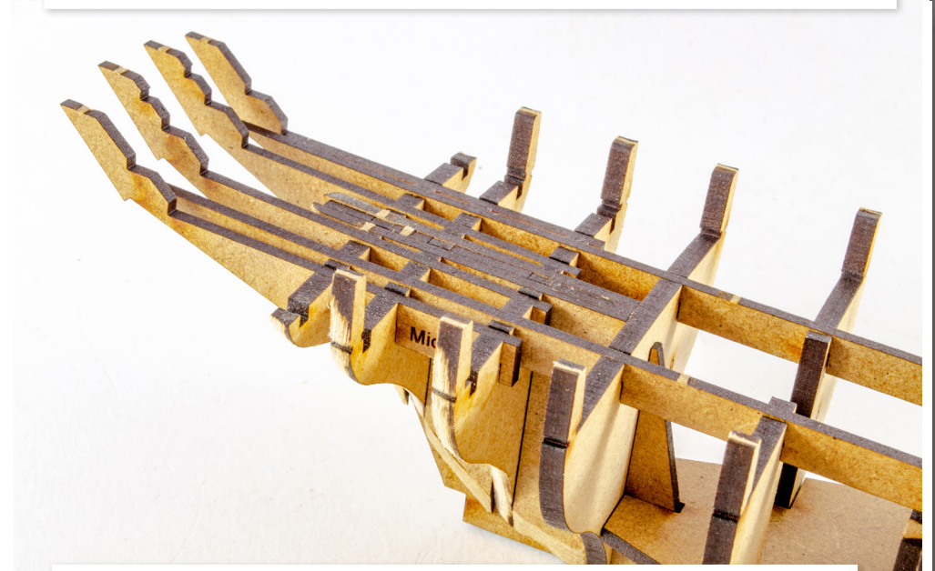
36. Dry fit (no glue) both parts to the outside of the previous pair, using the bulkhead slots.
