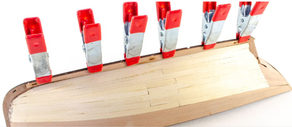
70. Glue part #48 into place along the keel so the locating slots perfectly align. Clamp until dry. You can now insert those pegs into the slots, using glue, and then glue/clamp the other part #48 onto the opposite side of the keel.
